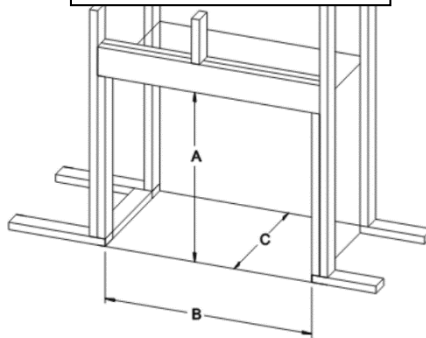
Framing Dimensions
